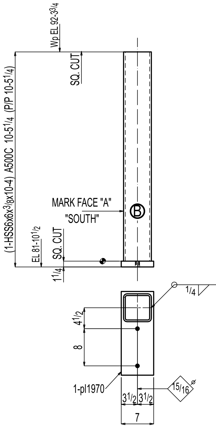
ONE COLUMN F-10.02C1
