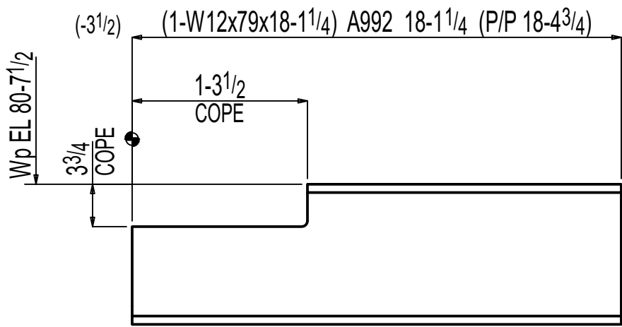
ONE BEAM F-10.02B1
