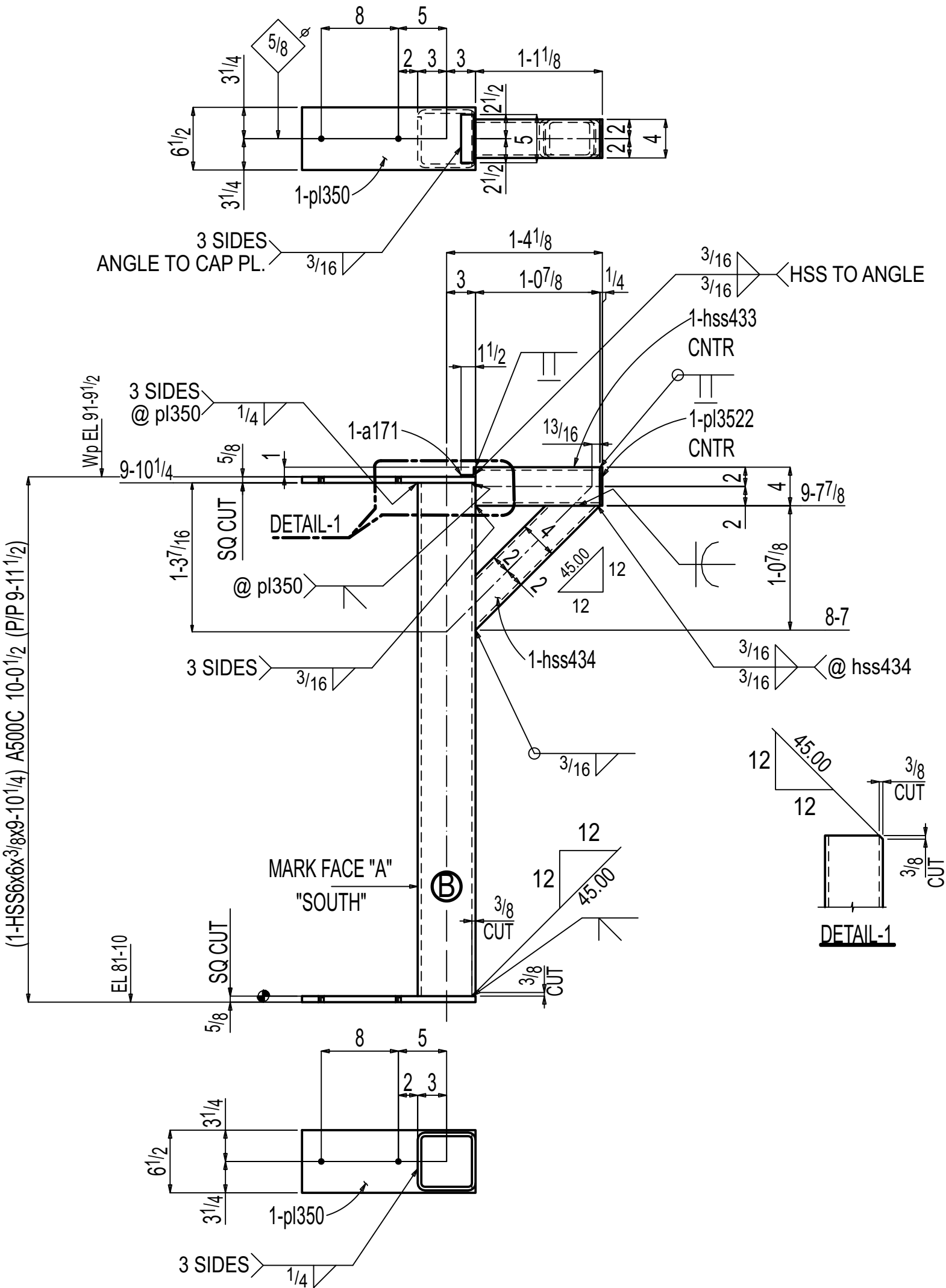
ONE COLUMN F-10.02C2
